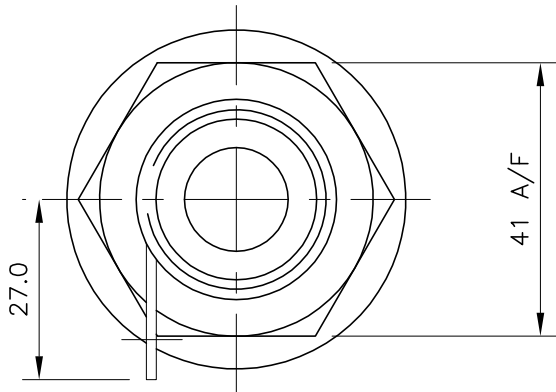
VIEW IN DIRECTION OF ARROW 'X'
