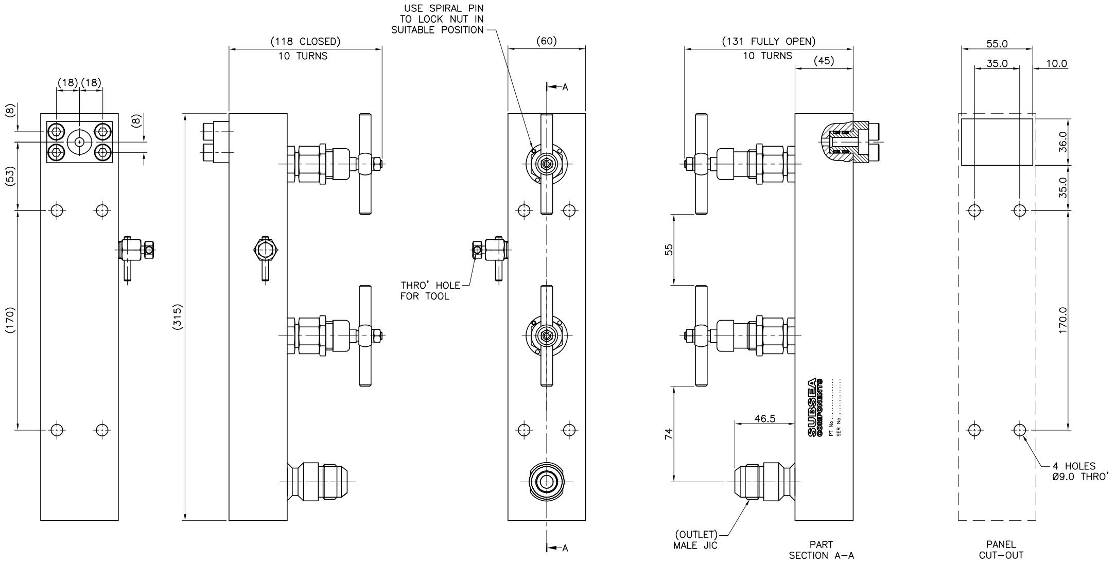
GA DOUBLE BLOCK & BLEED MANIFOLD SEAL SUB INPUT-MALE JIC OUTLET (MWP 690 BAR)
