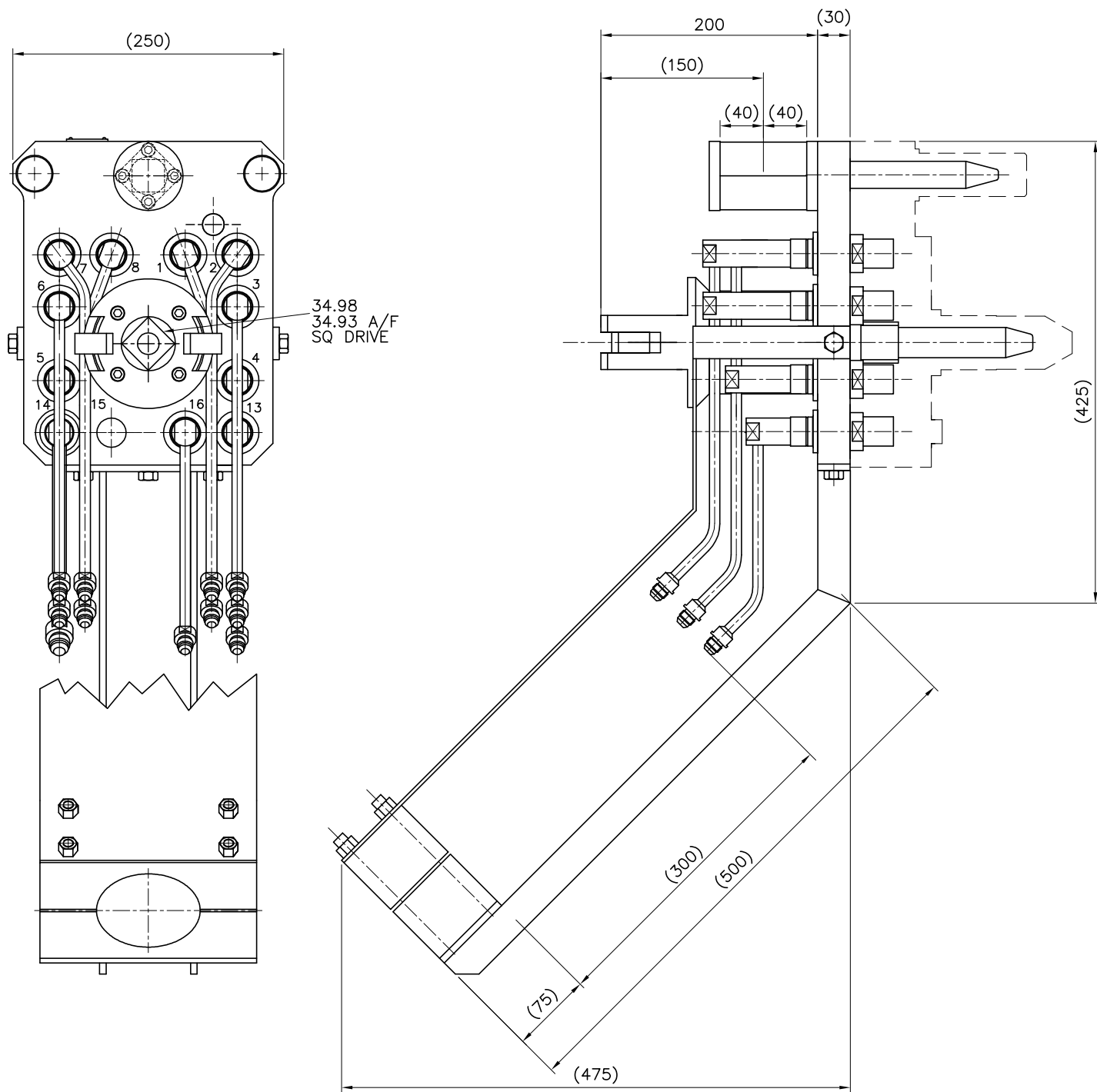
GA - FEMALE ROV STABPLATE (17-H) - 12 WAY (11 POP)
